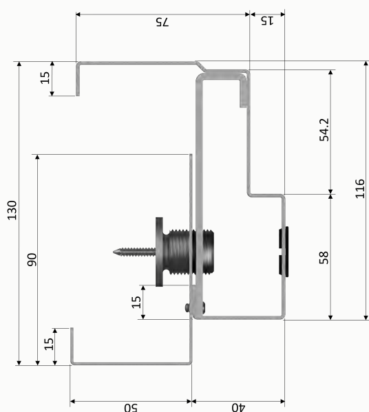
Outward Header & Hinge Profile
