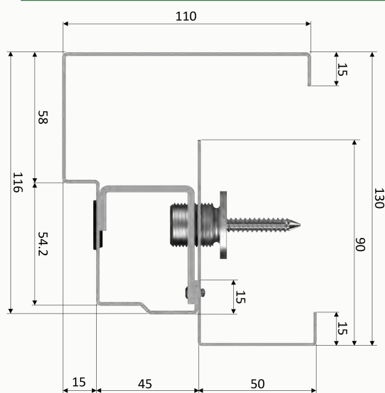
Inward Strike Profile
