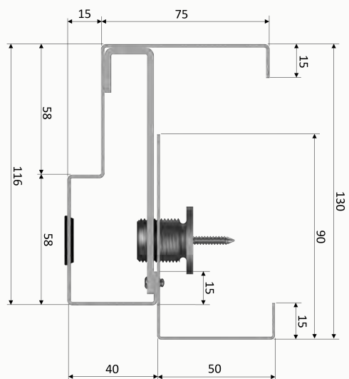
Outward Strike Profile
